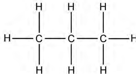
propane
